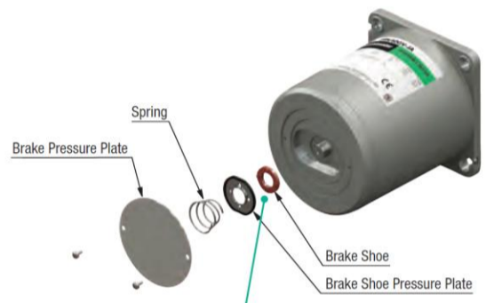
Brake Shoe: Uses a material excellent in abrasion resistance
