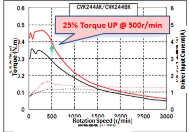
2 Phase Bipolar □42mm
