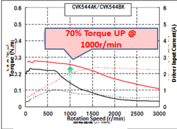
5 Phase □42mm
